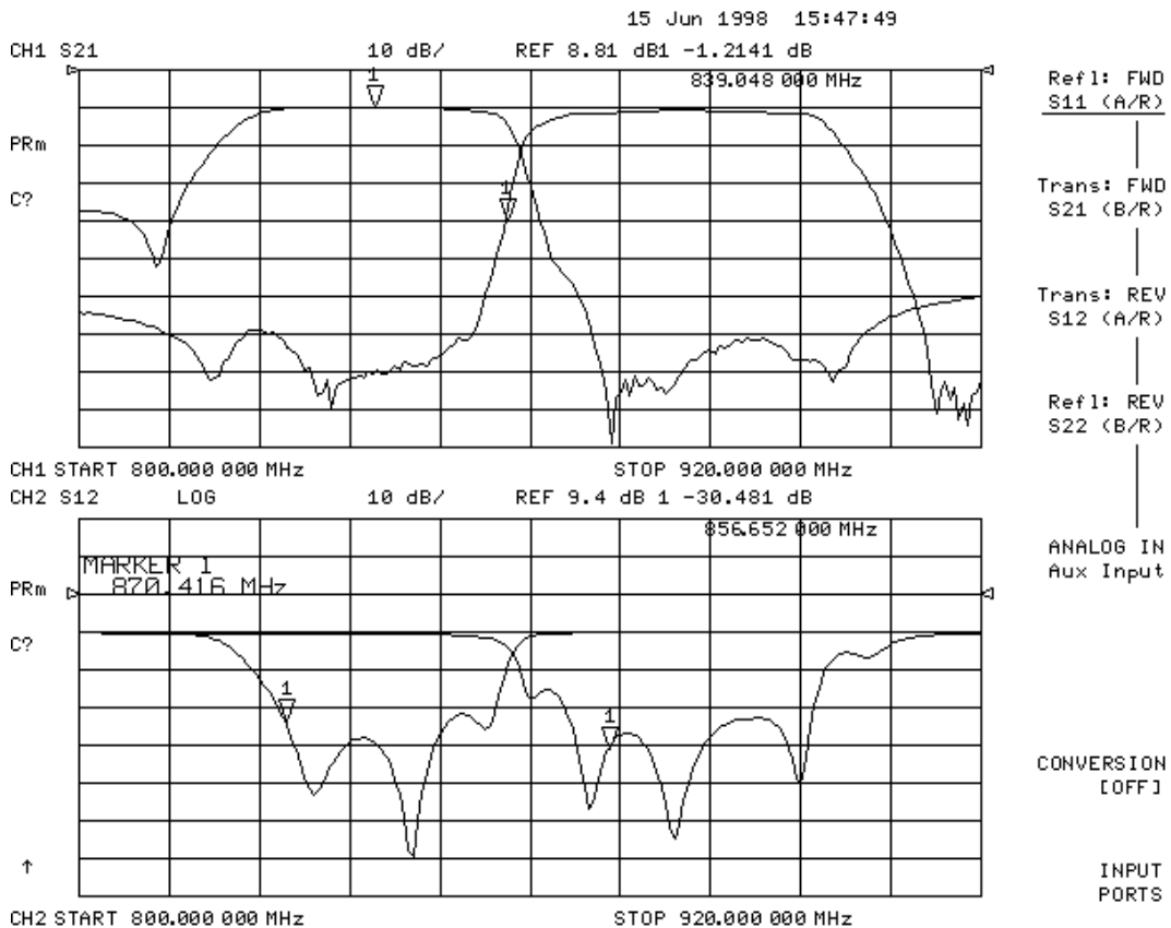
Figure 4. Duplexer Measurement
