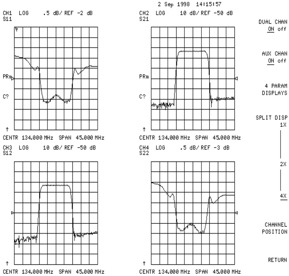
Figure 3. Four-Channel Display
